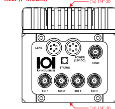
Rear (EF-Mount)
