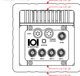
Rear (EF-Mount)
